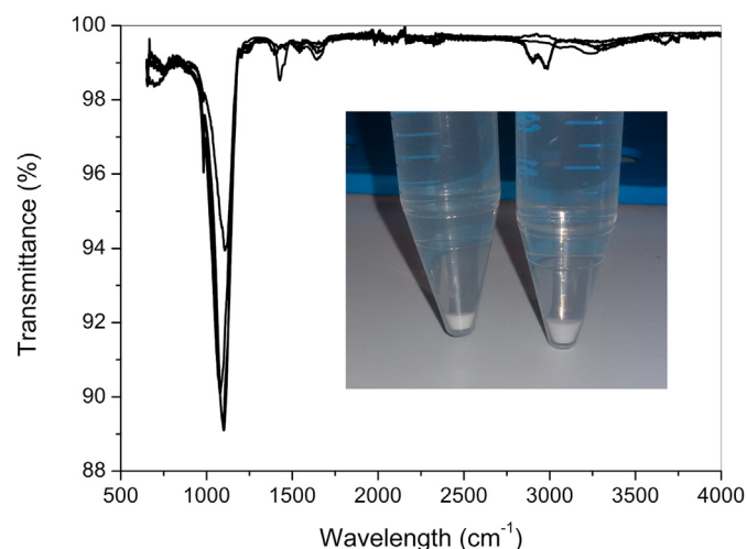
Fig. 5. FT-IR analysis of precipitates from glucose-limited chemostat cultures and a picture of the precipitates.
