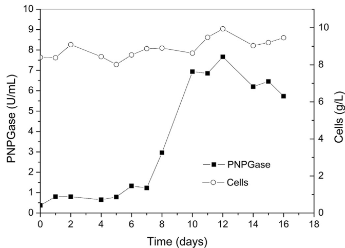
Fig. 4. Continuous PNPase production using glucose at 20 g/L (G202).
